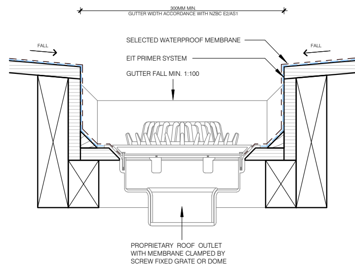
3 INTERNAL GUTTER WITH OUTLET 1:5
